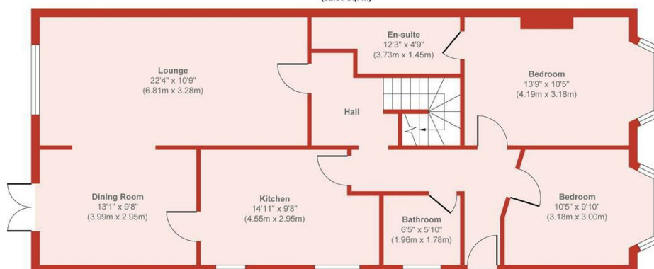
Ground Floor Approximate Floor Area 1043 sq. ft (96.89 sq. m)
