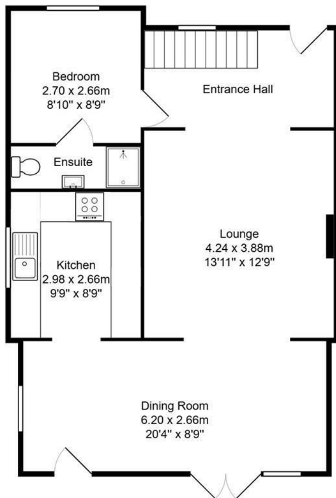
Ground Floor Area: 60.0 m 2 ... 645 ft 2
