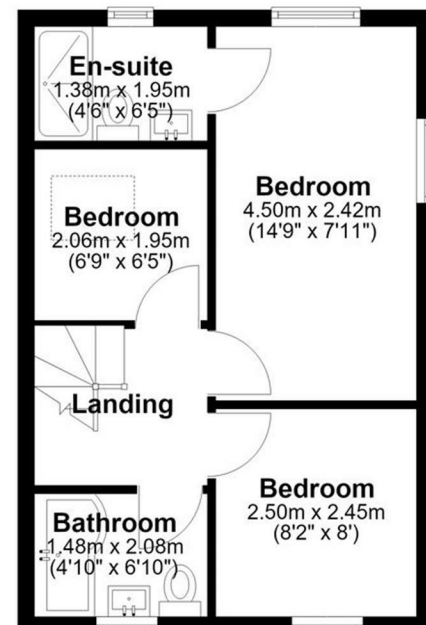
First Floor Approx. 32.3 sq. metres (347.5 sq. feet)
