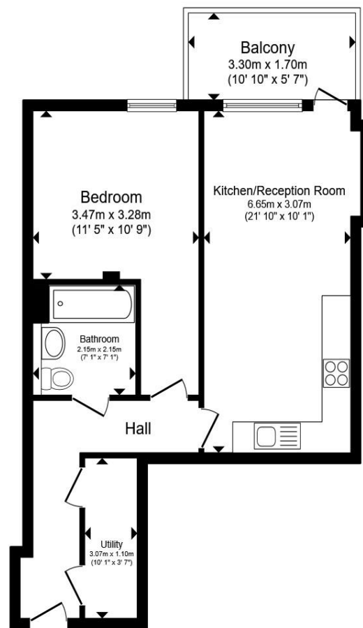
2nd Floor
