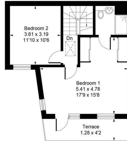
Second Floor
