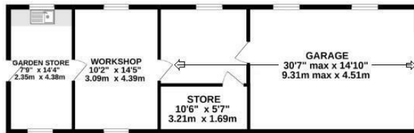
GROUND FLOOR 1917 sq.ft. (178.1 sq.m.) approx.
