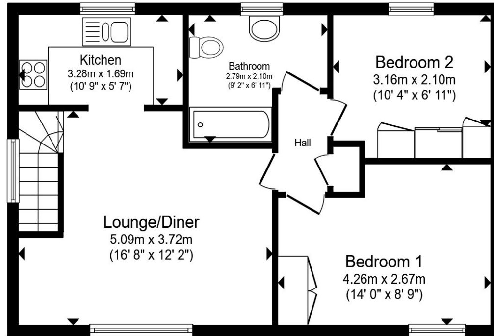
First Floor
