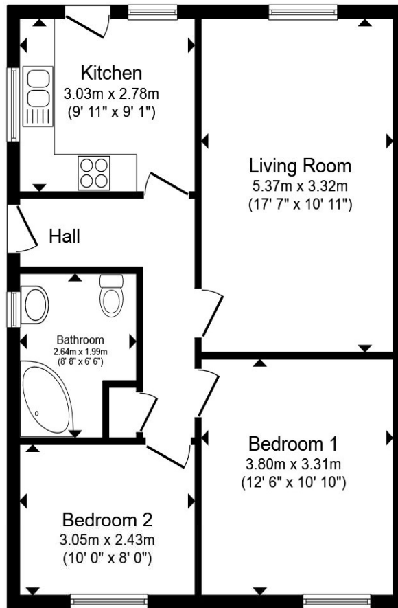
Floor Plan
