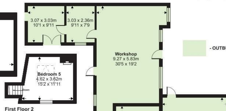
First Floor 2
