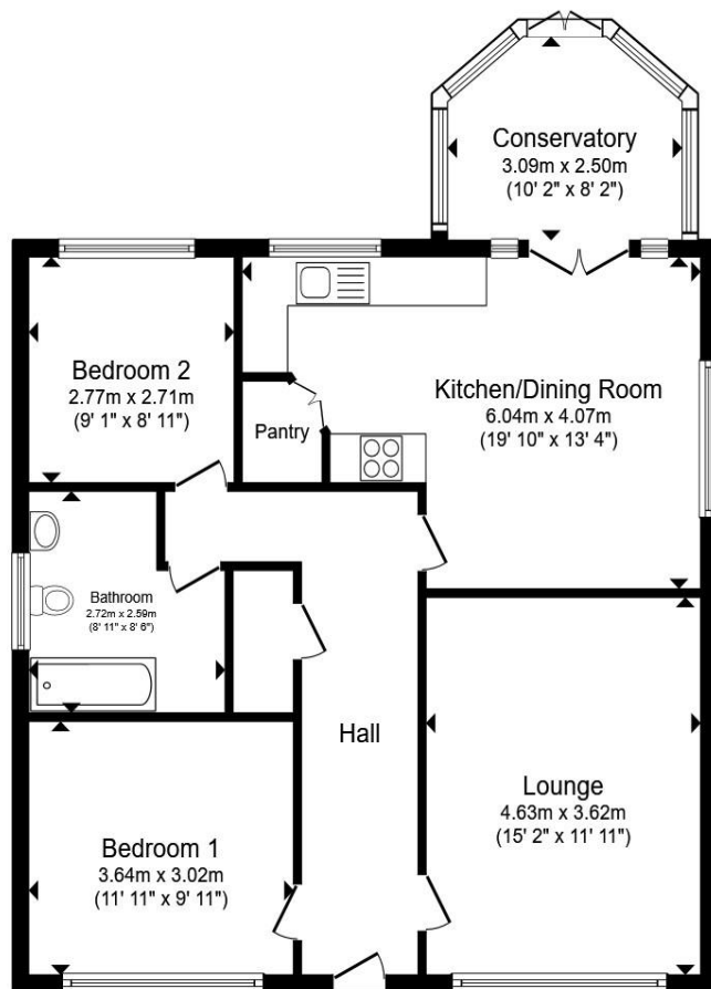
Floor Plan
