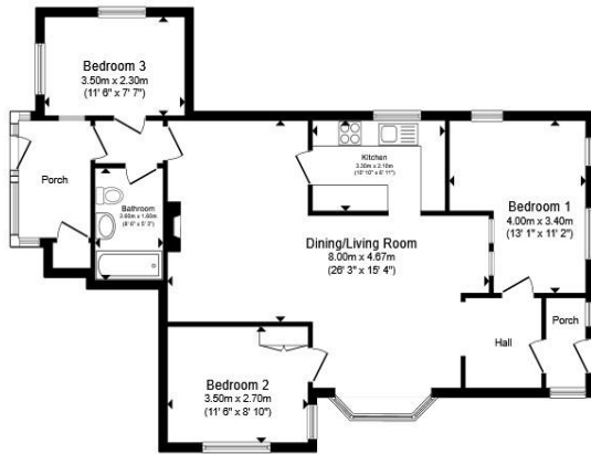
Floor Plan
