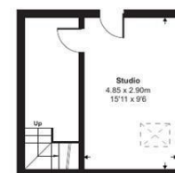
Annexe Ground Floor
