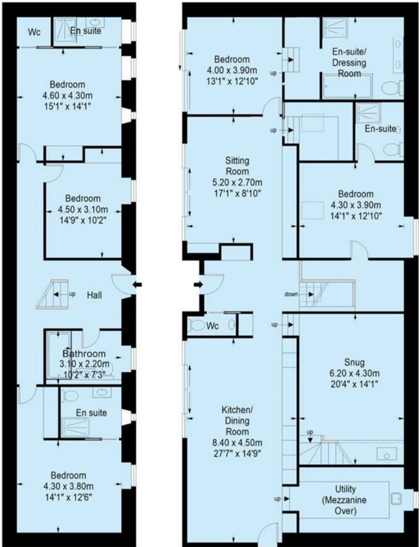
Ground Floor
