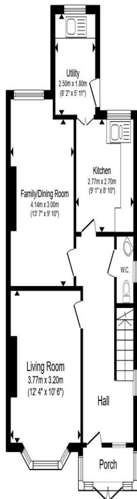
Ground Floor
