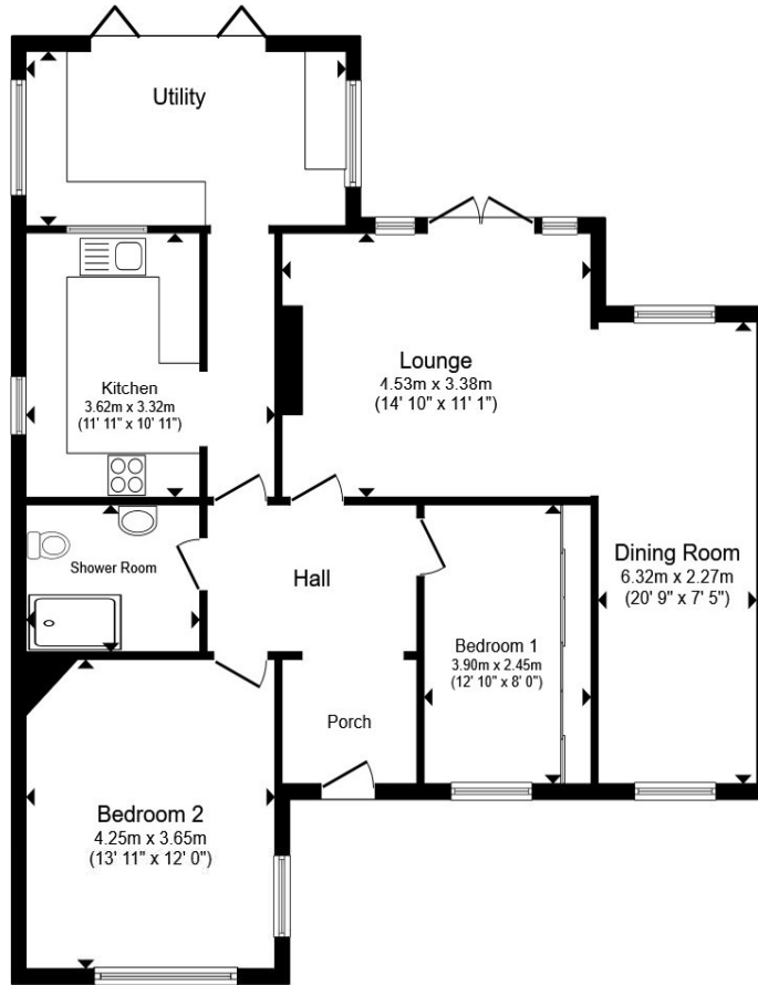
Floor Plan
