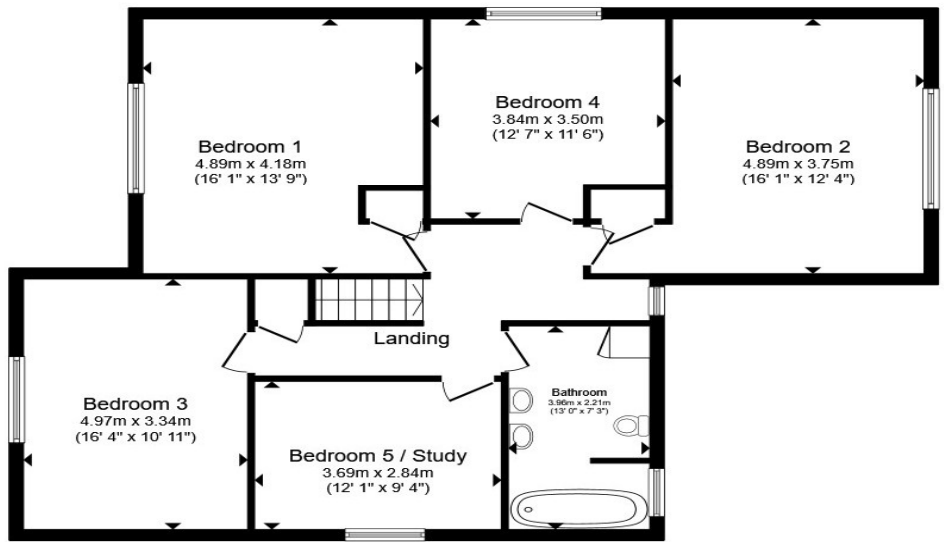
First Floor
