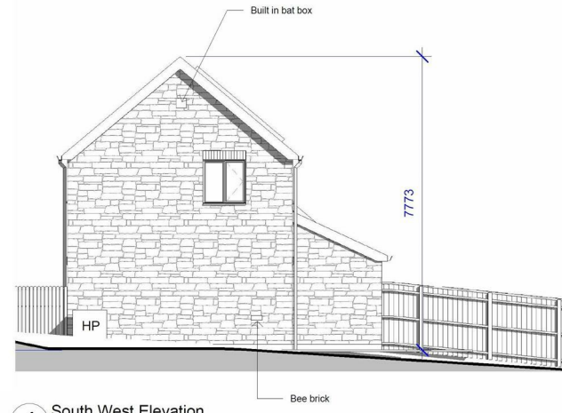
4 South West Elevation 1 : 100
