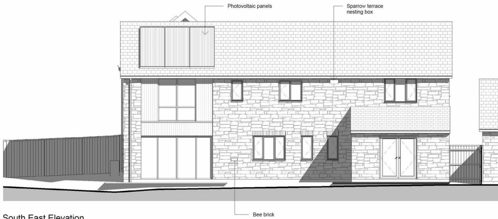
3 South East Elevation 1 : 100
