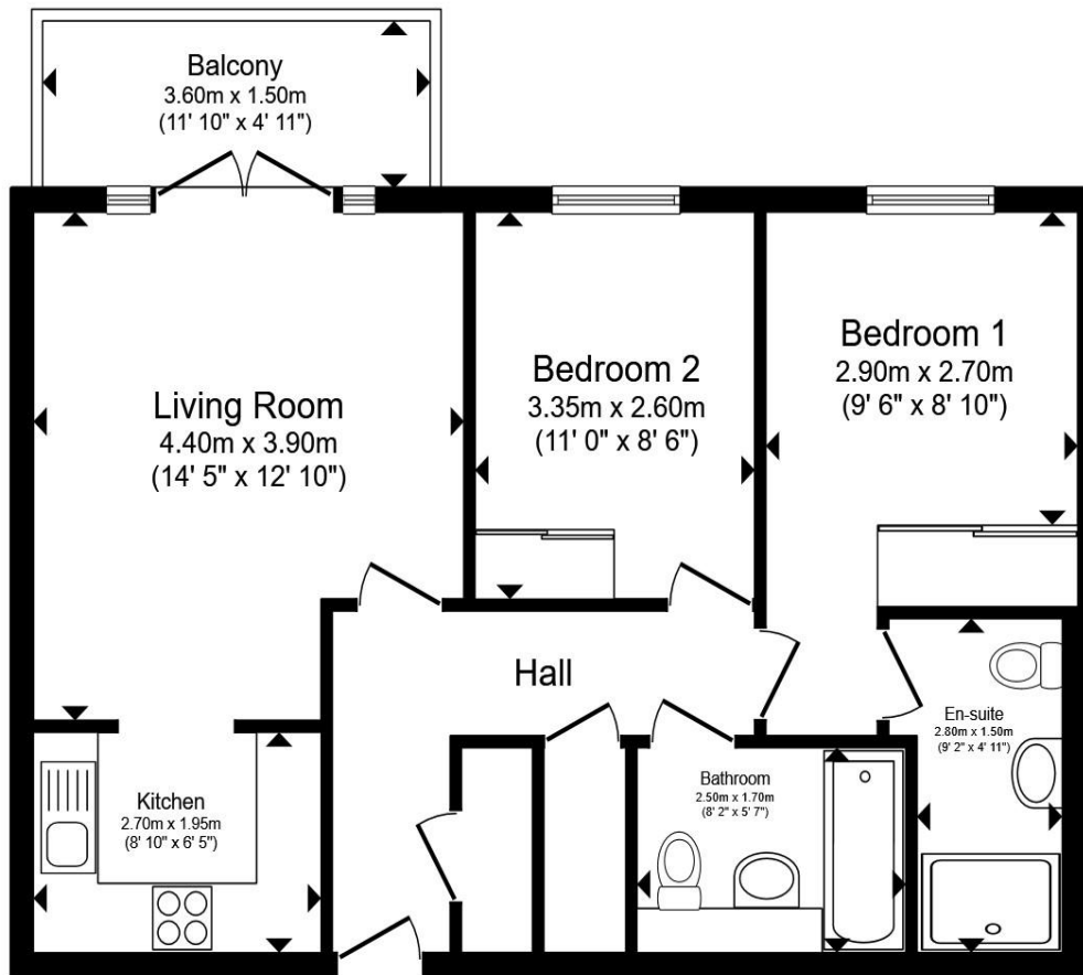
First Floor
