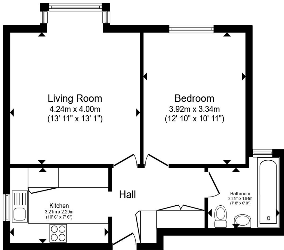
Floor Plan
